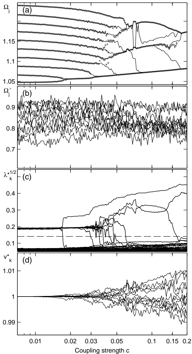
Figure 8. Same analysis as in Fig. 5 but the output of the oscillator chain being analyzed is contaminated by Gaussian noise of the same variance as the signal. (a) Estimated frequencies \Omega_j from rotated PCs (gray dots) and the observed frequencies \Omega_j from the noiseless case (solid lines); (b) observed frequencies \Omega'_j of the noise-perturbed case; (c) modified variances \lambda_k^* , k \leq 20 , along with the unchanged eigenvalues \lambda_k , k \geq 21 ; and (d) modified eigenvalues v_k^* of the phase coupling matrix.
