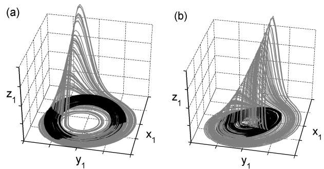
Figure 4. Reconstruction of the leading pair, i. e. RCs 1-2 (black curve), of the coupled Rössler oscillators' actual trajectory (gray curve) in (a) a phase-coherent regime with \alpha = 0.15 ; and (b) in the funnel regime with \alpha = 0.28 .
