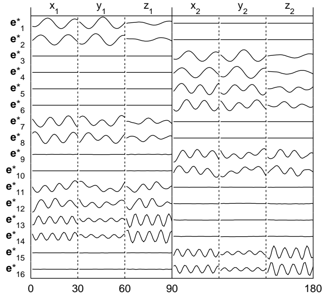
Figure 10. Rotated eigenvectors e_k^* associated with the 16 largest eigenvalues \lambda_k^* in Fig. 9.
