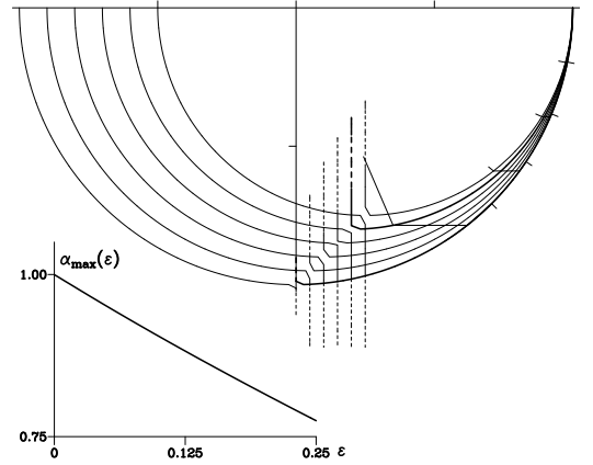
Figure 19. Complex roots for the LF-Asselin Filter time-stepping algorithm for \epsilon = 0, 0.05, 0.1, 0.15, 0.2, and 0.25 . The curves corresponding to \epsilon = 0 , and 0.2 are highlighted. The presence of \epsilon terms in (A.7) moves roots strictly along the real axis relative to unfiltered LF roots. \epsilon does not affect the imaginary part of \lambda_{\pm} as long as the expression under the radical is positive. Because of this feature, an Asselin filter causes an additional phase-lead error to an already forward-dispersive LF. The lower-left portion shows the dependency of the stability limit \alpha_{\max} on \epsilon ( cf. , (A.8)).
