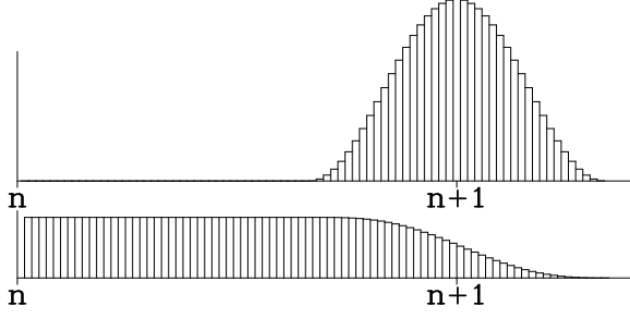
Figure 15. Structure of the fast-time-averaging filter. Top: primary weights, \{a_m\} , for computing \langle \zeta \rangle^{n+1} and \langle \bar{\mathbf{U}} \rangle^{n+1} ; and Bottom: corresponding secondary weights, \{b_m\} , to compute \langle \langle \bar{\mathbf{U}} \rangle \rangle^{n+\frac{1}{2}} . Small tickmarks symbolize the fast (barotropic) time steps, and large ones labeled by n and n+1 are the old and new baroclinic steps.
