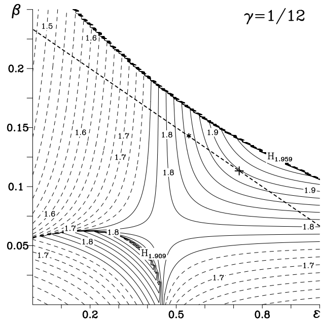
Figure 5. Top: Stability limit \alpha_{\max} as a function of \epsilon for algorithm (2.27)–(2.30) with \gamma = 1/12 for two different settings of \beta : (solid) along the line of vanishing \mathcal{O}(\alpha^5) term (2.36) and (dashed) \beta = 0 . Bottom: \alpha_{\max} as function of \epsilon, \beta with fixed \gamma = 1/12 . Contours below \alpha = 1.75 are shown in dashed lines. The empty area in the upper-right corner corresponds to schemes with an asymptotic instability of the physical modes. Note the appearance of two maxima of stability, at (\epsilon, \beta) = (0.83, 0.126) just on the edge of asymptotic instability, and (0.39, 0.044) . The straight dashed line approximately parallel to the edge corresponds to a zero \mathcal{O}(\alpha^5) truncation term. The asterisk * and cross + on this line denote locations of the minimal truncation error and maximum stability limit among the forth-order algorithms.
