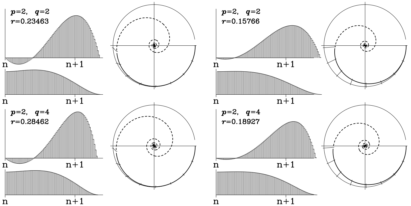
Figure 17. Shape functions and corresponding step multipliers \lambda(\alpha) for the filter (3.64) with different choices for p and q . (Left side): second-order accurate filters; (right side): optimized for minimal numerical dispersion (3.59).
