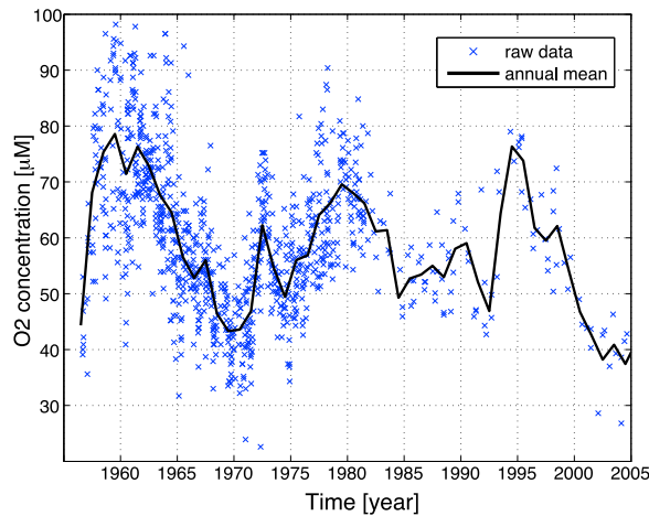
Figure 2. Time series of dissolved O_2 at Station Papa [Whitney et al. , 2007] in the subarctic North Pacific (50N, 145W). O_2 concentrations have been interpolated to the density surface \sigma_0 = 27.0 . The black solid line is the annually averaged O_2 , and the blue crosses are the individual measurements.
