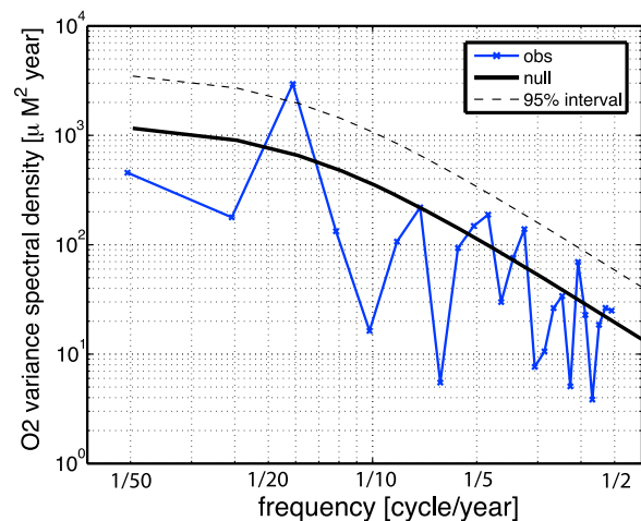
Figure 3. Periodogram of dissolved oxygen is plotted on the logarithmic scale (blue line), which is computed from detrended, annually averaged observations. The black solid line represents the null hypothesis predicted by the randomly forced simple model, and the thin, black dash line is the 95% confidence interval.
