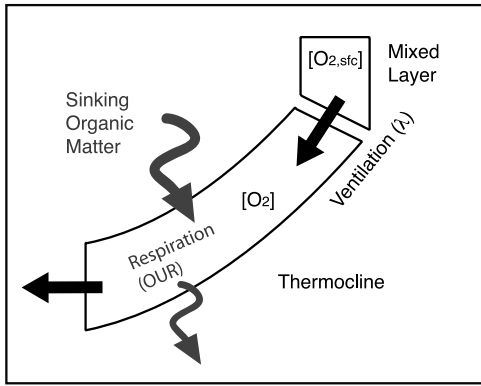
Figure 1. A schematic diagram of the oxygen cycle associated with thermocline ventilation. The thick solid arrows represent physical transport, and the wiggly grey arrows represent the flux of sinking organic matter. The convergence of physical transport balances the sink due to the respiration of the organic matter.
