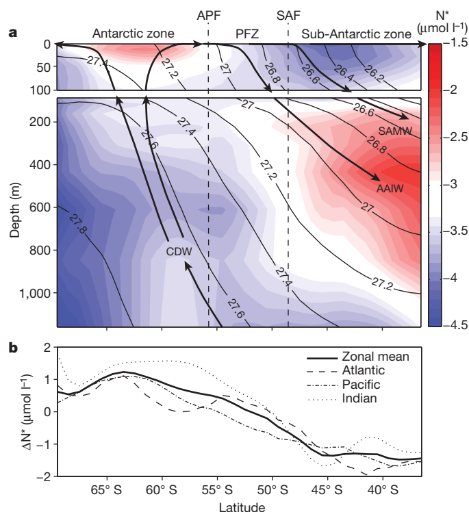
Figure 1 | Observed N^* distribution in the Southern Ocean. a, Zonal mean section of N^* ( [\text{NO}_3^-] - 16[\text{PO}_4^{3-}] ), with potential density contours ( \rho_\theta - 1,000 \text{ kg m}^{-3} ; thin lines) and schematic large-scale meridional overturning circulation patterns (arrows). Upwelling circumpolar deep water (CDW) is driven across the Antarctic polar front (APF) and the sub-Antarctic front (SAF) by Ekman transport, and subsides in the polar frontal zone (PFZ) to form Antarctic intermediate water (AAIW) and sub-Antarctic mode water (SAMW). b, Zonal mean vertical difference in N^* between the surface and the thermocline ( \Delta N^* = N^*_{0-75 \text{ m}} - N^*_{200-800 \text{ m}} ), globally and in individual sectors of the Southern Ocean.
