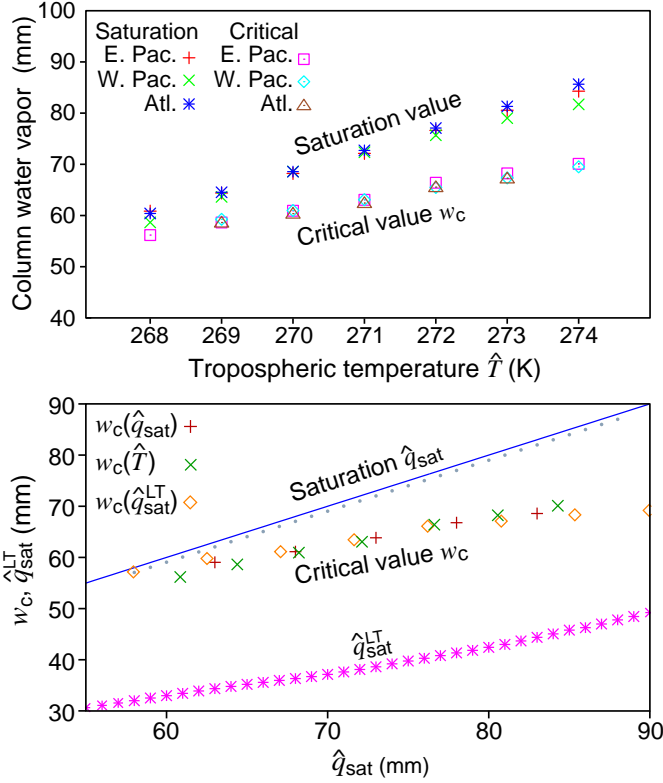
FIG. 3. (a) Critical column water vapor w_c and vertically integrated saturation water vapor \widehat{q}_{sat} as a function of tropospheric temperature \hat{T} for all basins. (b) As in (a), but for the critical value w_c determined as a function of \widehat{q}_{sat} , \widehat{q}_{sat}^{LT} and \hat{T} for the Eastern Pacific. Values of w_c(\hat{T}) [repeated from (a)] are plotted at the values of \widehat{q}_{sat} that correspond to \hat{T} = 268\text{--}274 K in that figure. Similarly, w_c(\widehat{q}_{sat}^{LT}) is plotted at \widehat{q}_{sat} values corresponding to \widehat{q}_{sat}^{LT} binned by \widehat{q}_{sat} (pink stars). The blue line shows \widehat{q}_{sat} for reference. Blue dots show \widehat{q}_{sat}^{ice} (using saturation with respect to ice).
