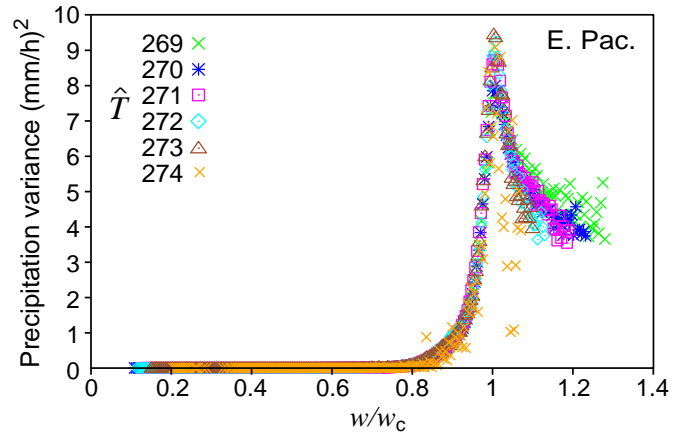
FIG. 4. Variance of precipitation conditioned on w in the Eastern Pacific, showing the collapse of the curves for all \widehat{T} when column water vapor is rescaled by the critical value w_c for each \widehat{T} .
