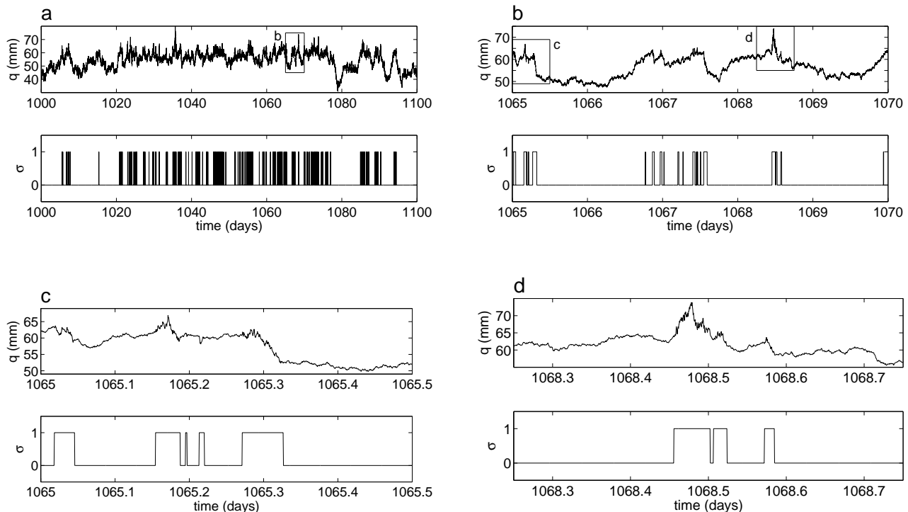
FIG. 2. Sample time series of q(t) and \sigma(t) . Temporal variations are shown over intervals of (a) 100 days, (b) 5 days, (c) 0.5 days, and (d) 0.5 days. The box in (a) shows the data used in (b), and the two boxes in (b) show the data used in (c) and (d). Compare (b) with the observational data in Fig. 2 of Holloway and Neelin (2010).
