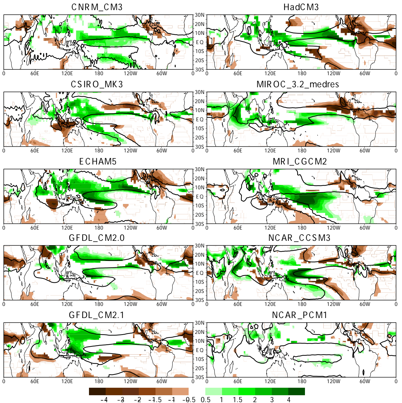
Fig. 8. Precipitation change in the JJA season for 2070–2099 relative to 1901–1960 ( \text{mm day}^{-1} ) from 10 ocean-atmosphere climate models for the SRES A2 global warming scenario. Values are shown only where they exceed the 95% confidence interval for a two-sided Student t test. The variance for the test is estimated at each point in the approximation that 10-year intervals in the control run are independent. One ensemble member is shown for each model because ensemble size varies from 1 to 5. For these 30-year mean values ensemble members bear close resemblance; for instance, for NCAR-CCSM3 spatial correlations of one ensemble member to another all exceed 0.95. The 4 \text{ mm day}^{-1} contour interval from the 1901–1960 base period is shown for each model.
