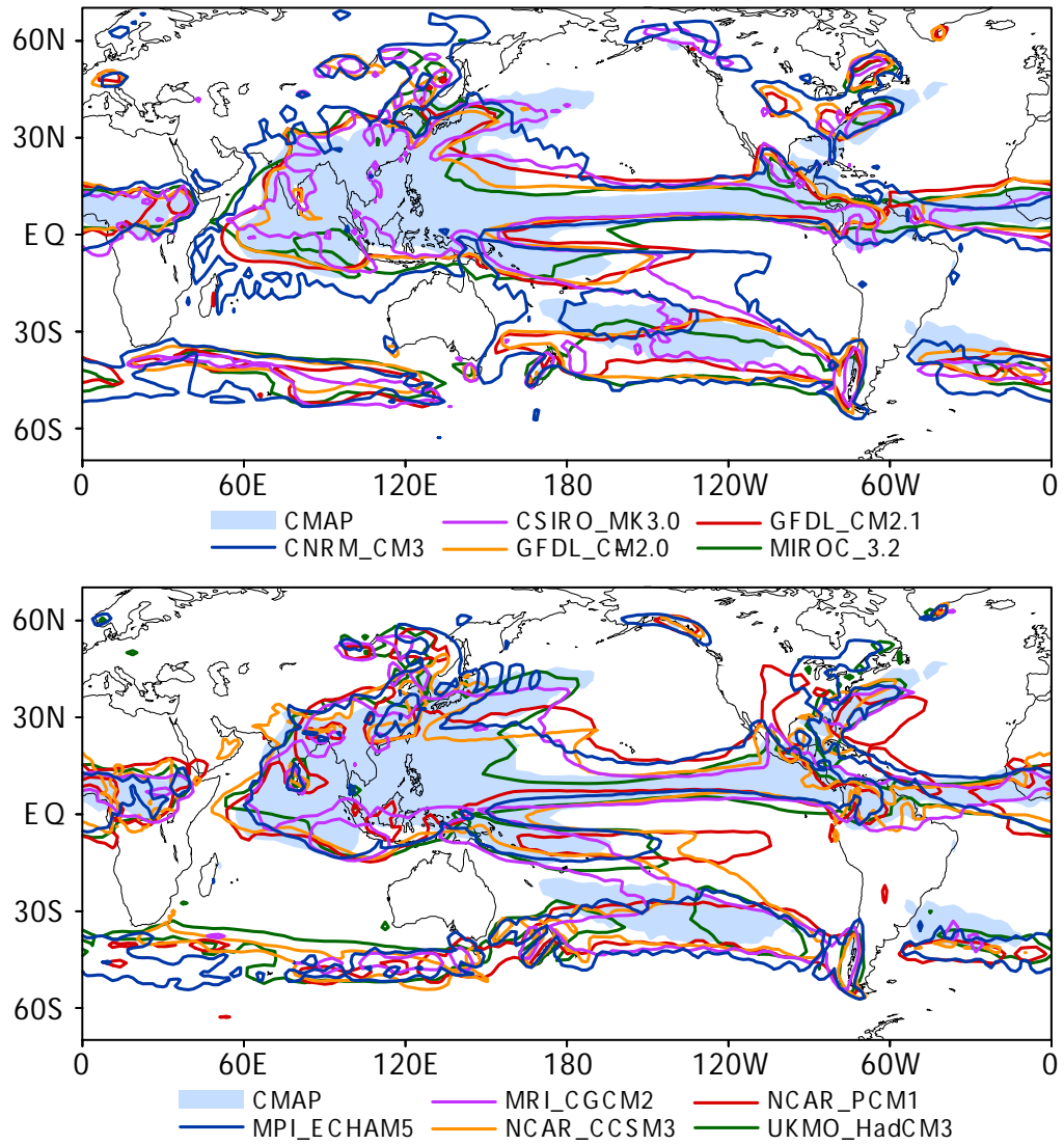
Fig. 7. Climatology of precipitation as summarized by the 4 mm day -1 contour line for JJA for each model (contour colors noted in key) and CMAP observations (blue shading over 4 mm day -1 ). The JJA average of 1979–2000 is used because of the availability of observations.
