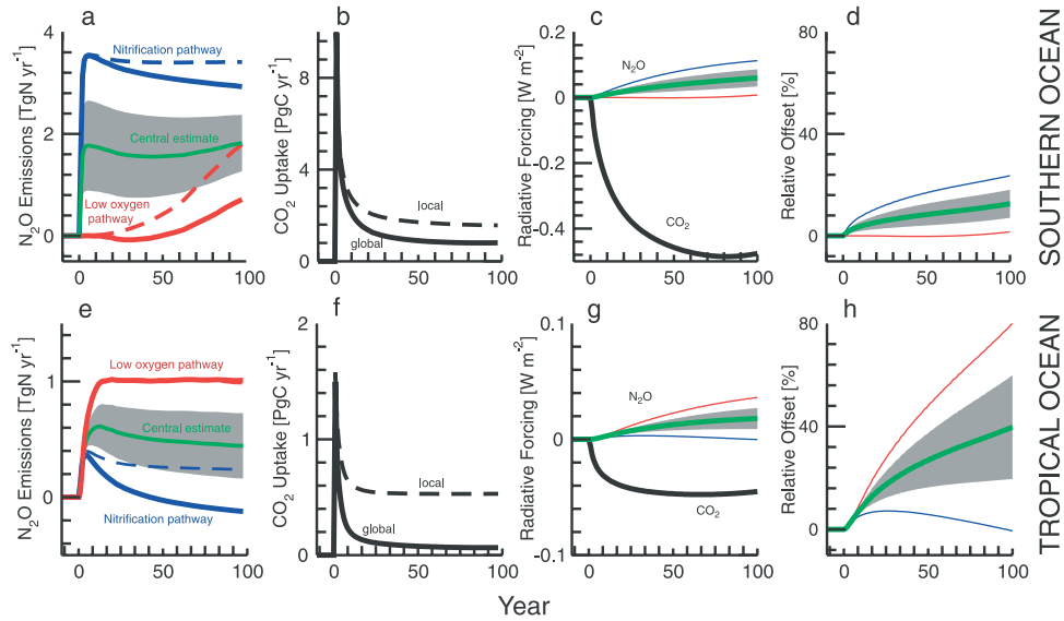
Figure 1. Time series of the response of oceanic and atmospheric \text{N}_2\text{O} and \text{CO}_2 to long-term (100yr) and large-scale fertilizations. Shown are the changes in response to fertilization (a–d) in the Southern Ocean (south of 31^\circ\text{S} ) and (e–h) in the Tropics ( 18^\circ\text{S} – 18^\circ\text{N} ) relative to control simulations. (a) and (e): Fertilization induced \text{N}_2\text{O} emissions from the ocean surface. (b) and (f): Fertilization induced \text{CO}_2 uptake by the ocean surface. (c) and (g): Fertilization induced changes in atmospheric radiative forcing. (d) and (h): Magnitudes of the \text{N}_2\text{O} offsetting effect. The blue and red lines indicate the emissions induced by the nitrification and low oxygen pathways, respectively. The green line represents our central estimate, with the uncertainties indicated as a gray band. All solid lines show global changes, while the dashed lines represent the fluxes integrated over the fertilized areas only. The results are from the HiSo-Lo model.
