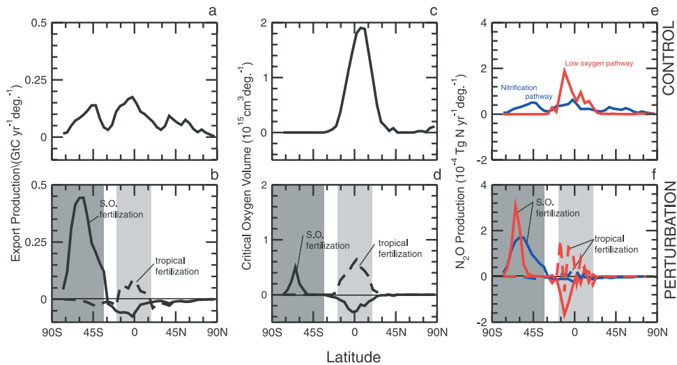
Figure 2. Plots of zonally integrated properties controlling the marine production of \text{N}_2\text{O} and their changes in response to fertilization. (a) Zonally integrated export production in the control simulation (without fertilization). (b) Changes in zonally integrated export production as a result of fertilization in the Southern Ocean (dark gray) and in the tropics (light gray). (c) Zonally integrated volume of water that has oxygen concentration lower than 50 \mu\text{mol kg}^{-1} , i.e., \text{O}_2 concentrations that give rise to a high yield of \text{N}_2\text{O} (d) Changes in the zonally integrated volume of water with critical oxygen concentrations. (e) Zonally and depth integrated production of \text{N}_2\text{O} by the nitrification (blue) and low oxygen (red) pathways. (f) Changes in the zonally and depth integrated \text{N}_2\text{O} production. The results are from the HiSo-Lo model.
