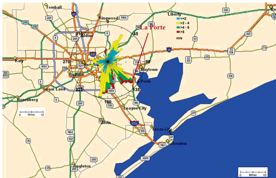
FIGURE 6. Windrose, Houston, TX, TEXAQS 2000 study period with the wind blowing to the center of the rose where the HRM-3 site is located. Note that one of the dominant wind vectors comes from the direction of La Porte, the location of the UCLA DOAS.
